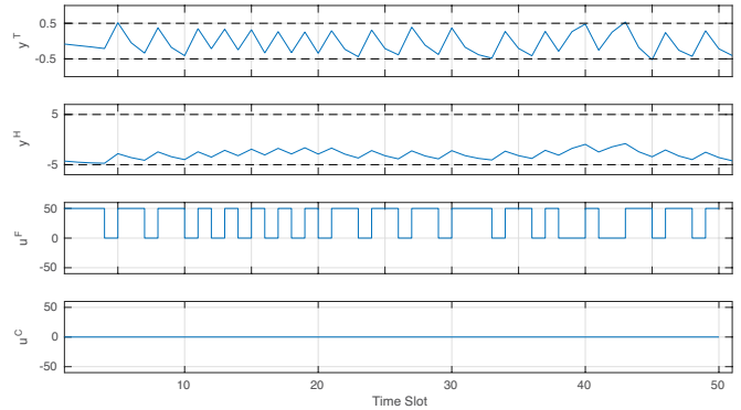
Fig. 2. Proposed chance-constrained approach.
