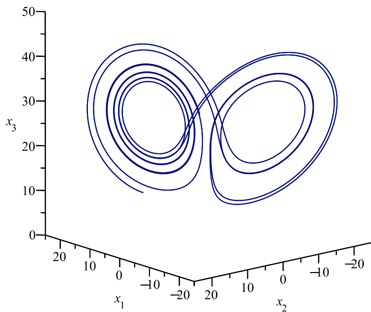
Figure 4: Simulation of the exact nonlinear Lorenz attractor
