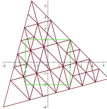
Figure 1: Regular edge bisection method for simplicial decomposition. Green lines denote the domain of interest, and the brown lines show the simplicial decomposition.
