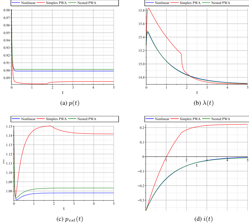
Figure 2: State trajectories comparison. For M_{\text{simplex}}^{\text{PWA}}, N_{\text{max}} = 500 , for M_{\text{nested}}^{\text{PWA}}, \delta = 0.01 .
