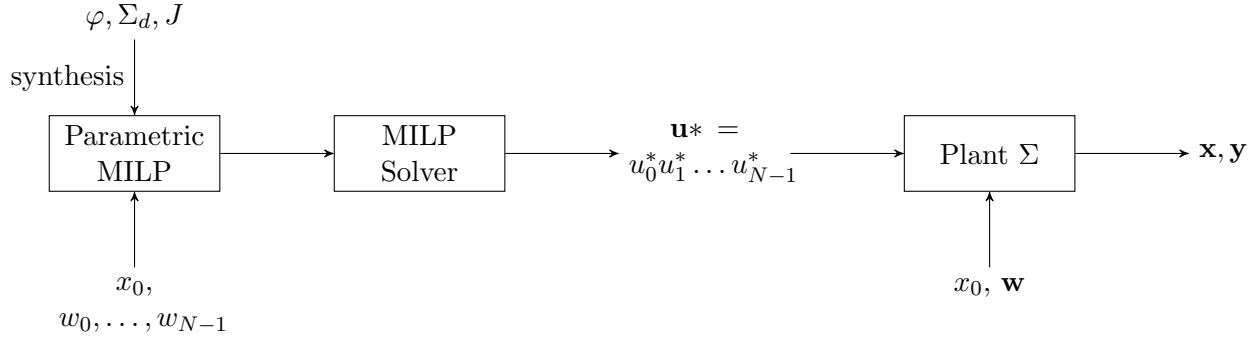
Figure 1: Open Loop Scenario. A parametric Mixed-Integer Linear Program is generated from the STL formula \phi , the discrete-time plant model \Sigma_d and the cost function J . The parameters of this MILP are the initial state x_0 and disturbance vector \mathbf{w} . When those are provided, a solver can compute an optimal solution \mathbf{u}^* for horizon N which is passed and used by the plant \Sigma .
