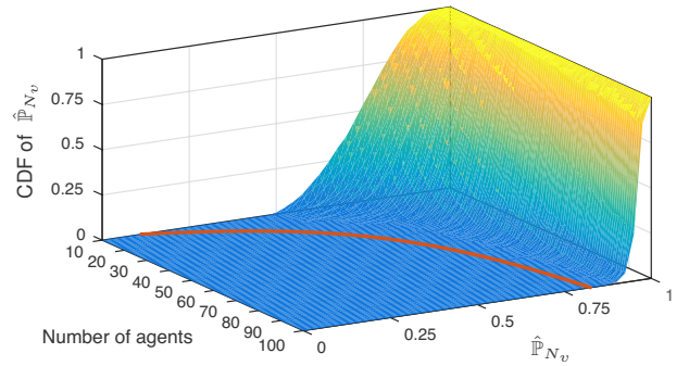
Fig. 2. Empirical Cumulative Distribution Function (CDF) of \hat{\mathbb{P}}_{N_v}\{x_{m,\delta}^* = (x_m^*, 0)\} over 1000 trials (surface) and theoretical bound 1 - \varepsilon_m (red line), both as a function of the number of agents m .
