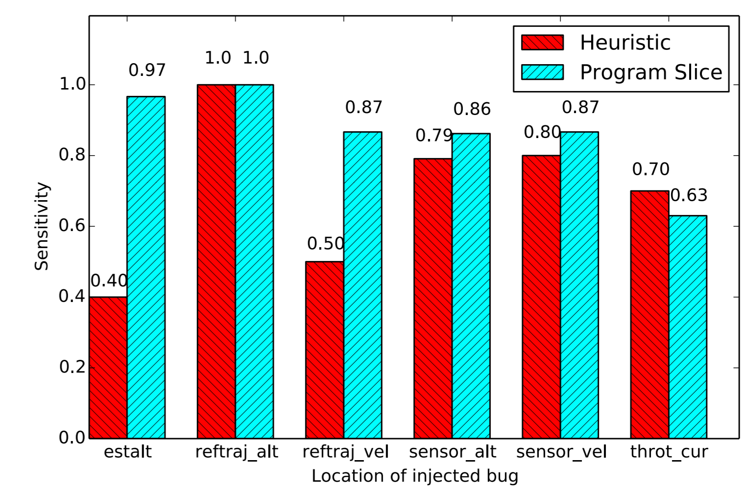
Figure 3. Sensitivities of both heuristic and program slice detectors for the six local variables where bugs were injected (higher is better). While the program slice performs better across four of the six variables, it does not always perform better. The program slice detector actually performs slightly worse for throt_cur and ties for reftraj_alt. For all the bug injection sites, the specificity was set to 0.8.
