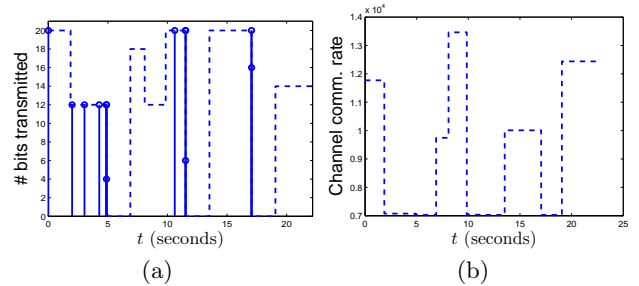
Fig. 1. (a) shows the transmission times, the number of bits transmitted on each transmission and the time-varying function n\bar{p} (dashed line). The three intervals, (4.88, 6.88] , (11.52, 13.52] and (17.05, 19.05] , with \bar{p} = 0 are the blackouts. (b) shows the time-varying function R .
