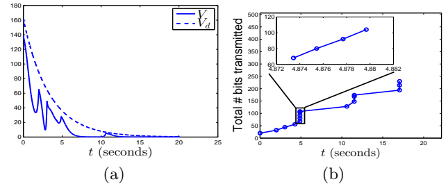
Fig. 2. Evolution of (a) V and V_d and (b) total number of bits transmitted, the inset shows that the transmission times are separated.
