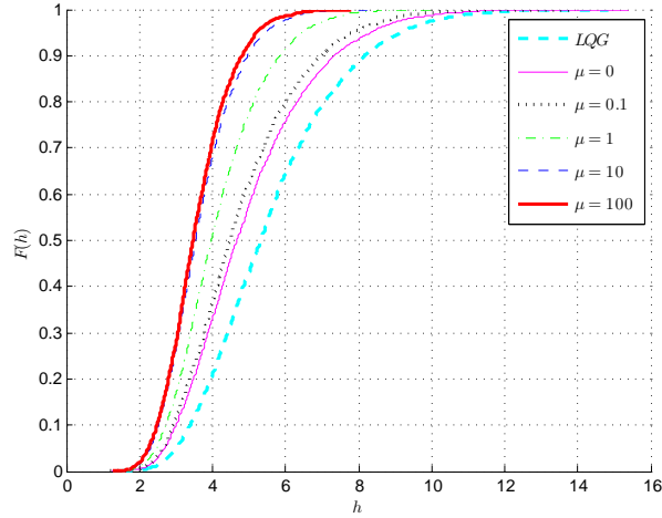
Figure 3: Probability distribution function of \|\mathbf{C}\mathbf{x}\|_\infty for the clipped controllers corresponding to the different values of \mu and for the clipped LQG controller.
