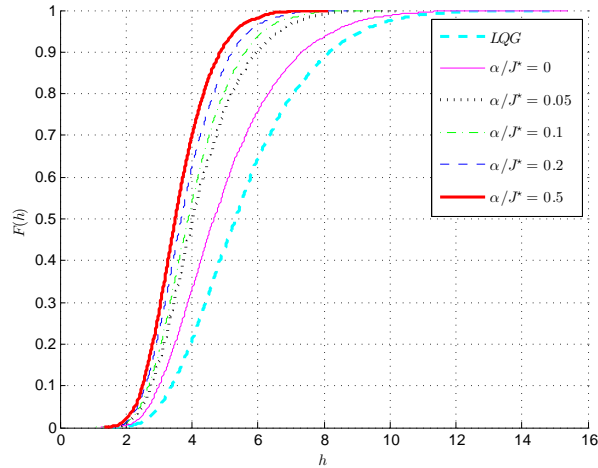
Figure 4: Probability distribution function of \|\mathbf{C}\mathbf{x}\|_\infty for the clipped controllers corresponding to the different values of \alpha and for the clipped LQG controller.
