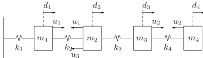
Figure 2: Scheme of the mechanical system.
