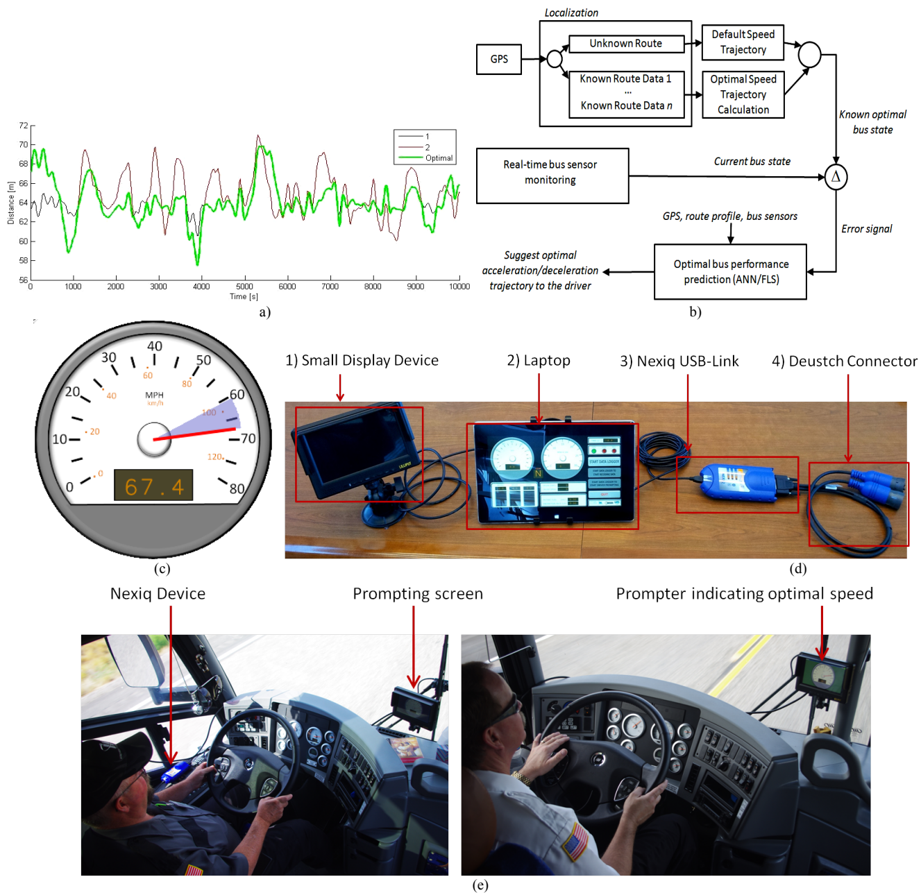
Fig. 1 a) optimal velocity trajectory. b) system architecture, c) System interface, d) vehicle fuel efficiency prompter, e) prompter sitting on a running vehicle
