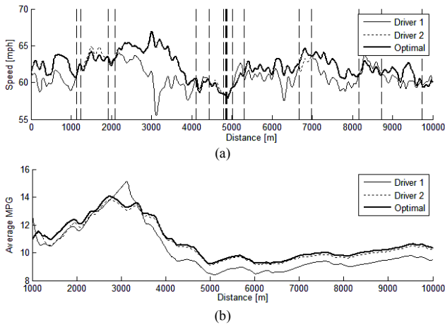
Fig. 9 Merged velocity profile with depicted switch points (dashed vertical lines) (a) and the resulting optimal MPG (b).
