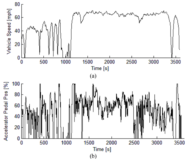
Fig. 2 Velocity (a) and gas pedal position (b) data recorder from a real bus.
