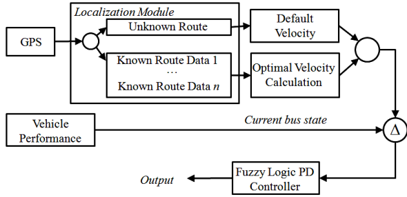
Fig. 1 Architecture of the proposed Intelligent Driver System.
