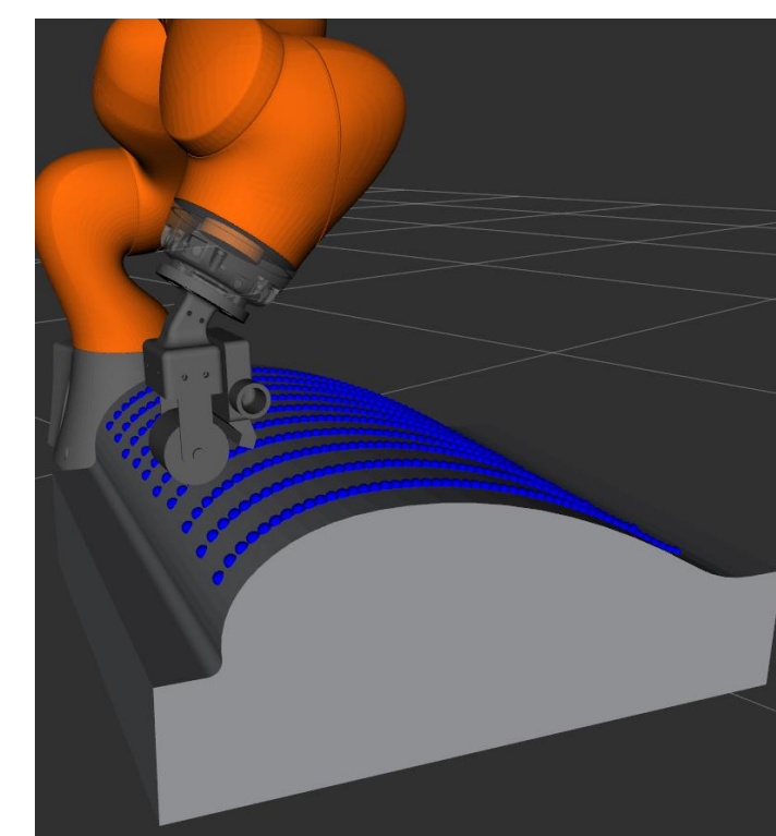
Draping robot executing paths under motion constraints in simulation
